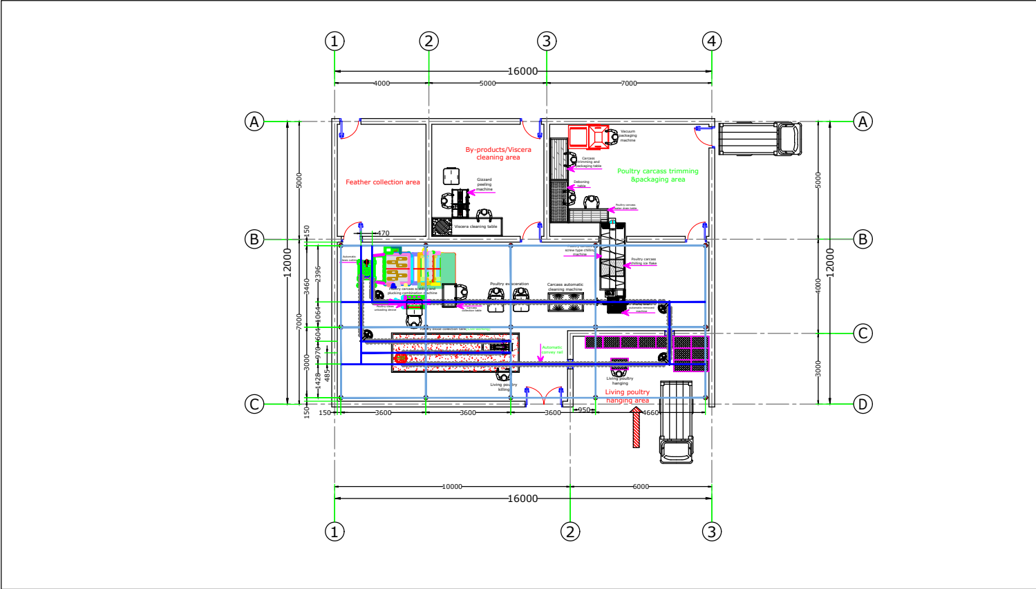
The 500 poultry per hour abattoir floor plan layout
